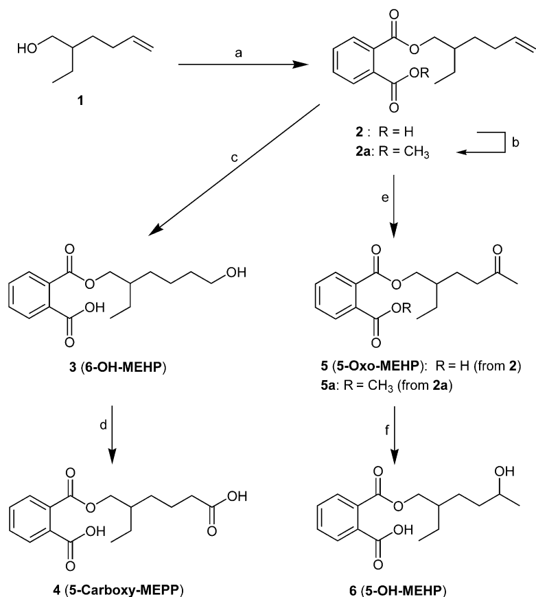
Scheme 1. Reagents and conditions: (a) phthalic anhydride, pyridine (Py), under N 2 ; (b) CH 2 N 2 , MeOH/ether (9:1); (c) 1 M B 2 H 6 in THF, then H 2 O 2 , OH − in THF; (d) CrO 3 , H 2 SO 4 in acetone; (e) PdCl 2 , quinone in DMF/H 2 O (7:1); (f) NaBH 4 in EtOH.
