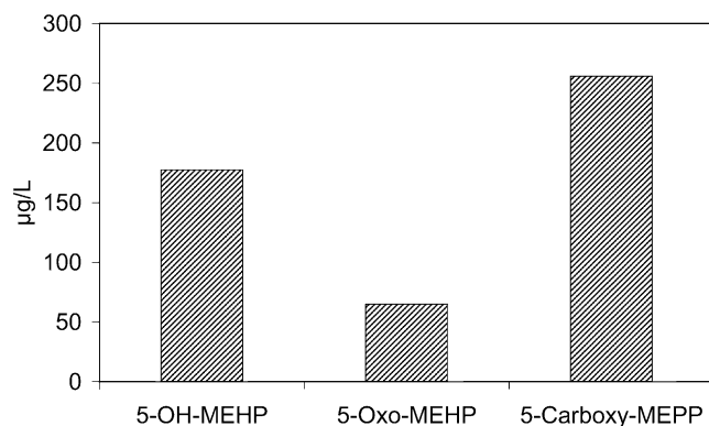
Figure 1. The concentrations of 5-OH-MEHP (6), 5-oxo-MEHP (5) and 5-carboxy-MEPP (4) in urine samples of 50 persons of the general population in µg/L. The 90th percentiles of these analytes, calculated assuming the underlying model to be a log-normal distribution, is shown.
